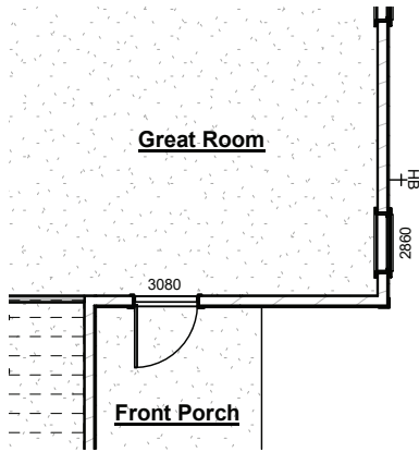
Great Room Door to Front Porch
