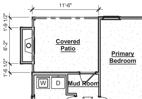
Outdoor Gas Log Fireplace with Cedar Mantel
