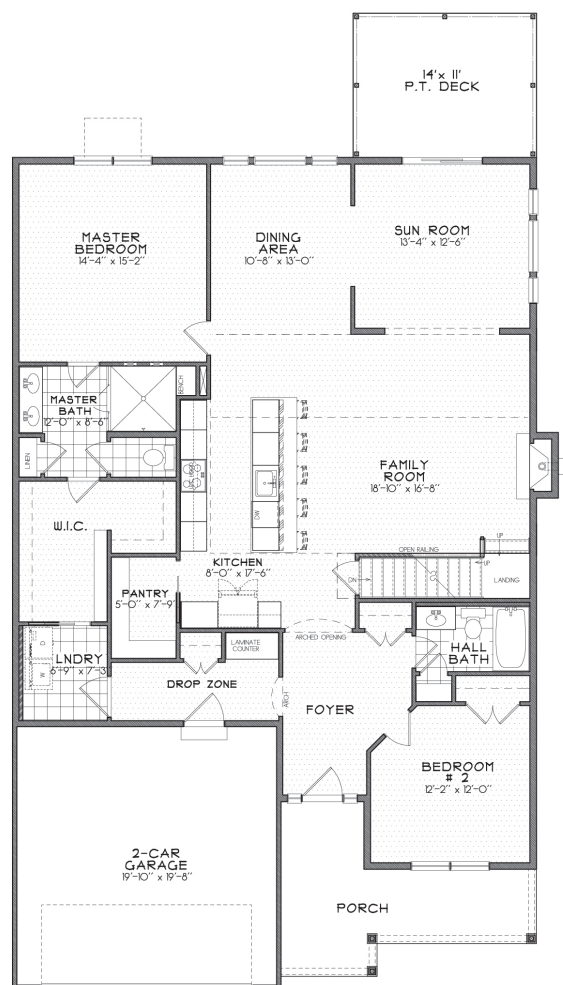
1,920 SQ. FT. FIRST FLOOR
