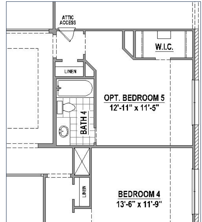
Bedroom 5 w/ Bath 4 (+297 SF)
