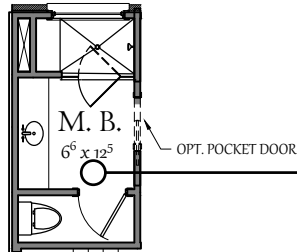
MASTER BATH LAYOUT- SUPER SHOWER OPTION
