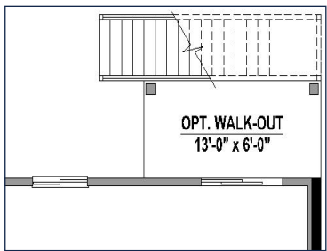
Basement Walkout with Deck Above
