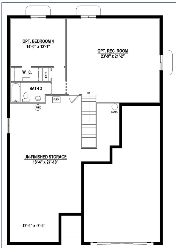
Rec Room w/ Bedroom 4 & Bath 3 (+934 SF)
