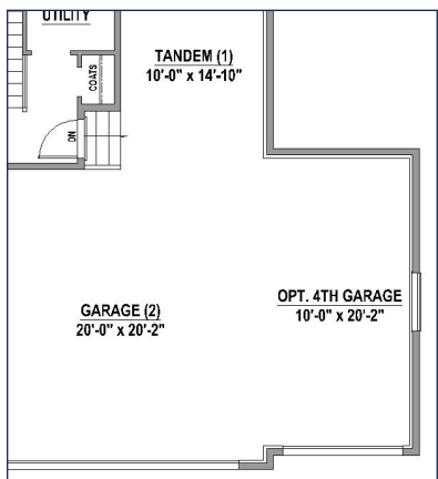
4th Car Garage
