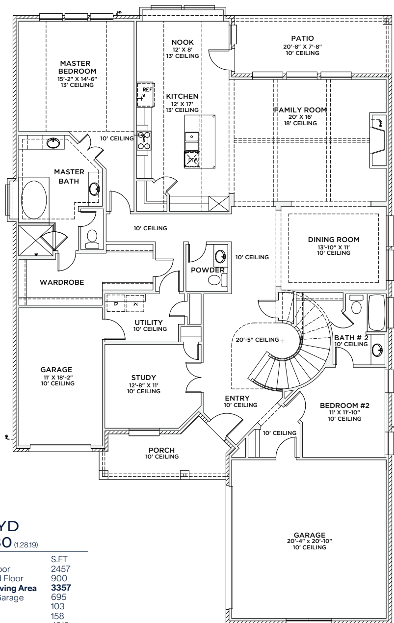
FIRST FLOOR
