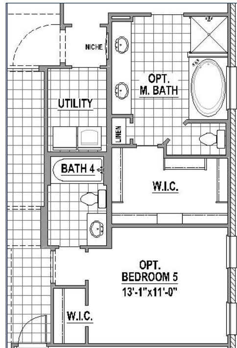
Alternate Main Bath & Bedroom 5
