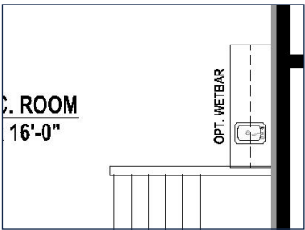
Optional Wet Bar in Rec Room
