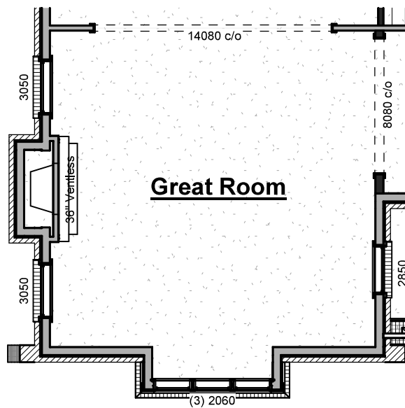
Great Room Fireplace Bump-Out
