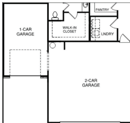
3-CAR FRONT ENTRY GARAGE
