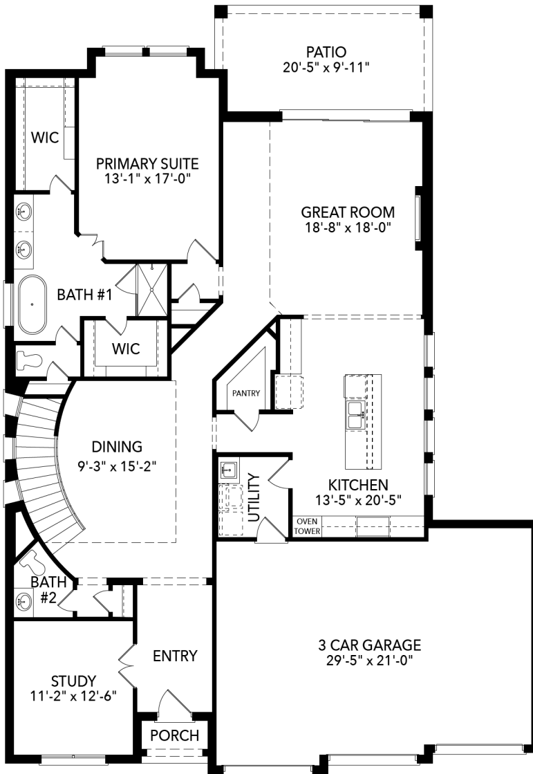
First Floor
