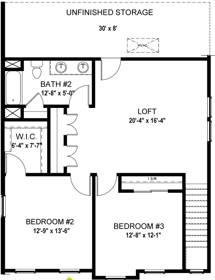
LOFT LEVEL
