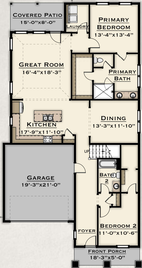
Main Level B
