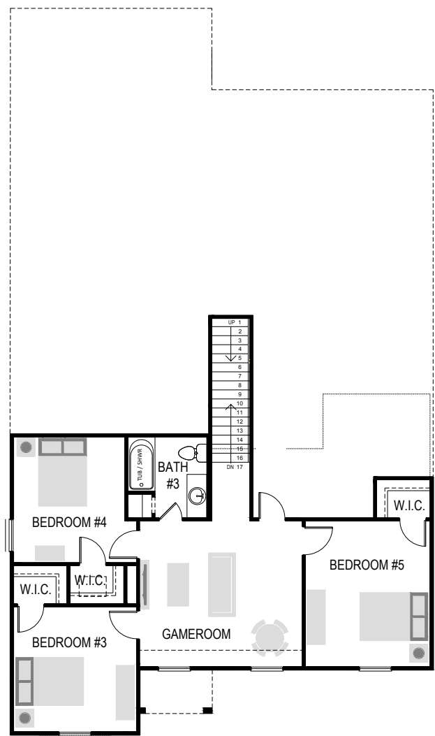
SECOND FLOOR
