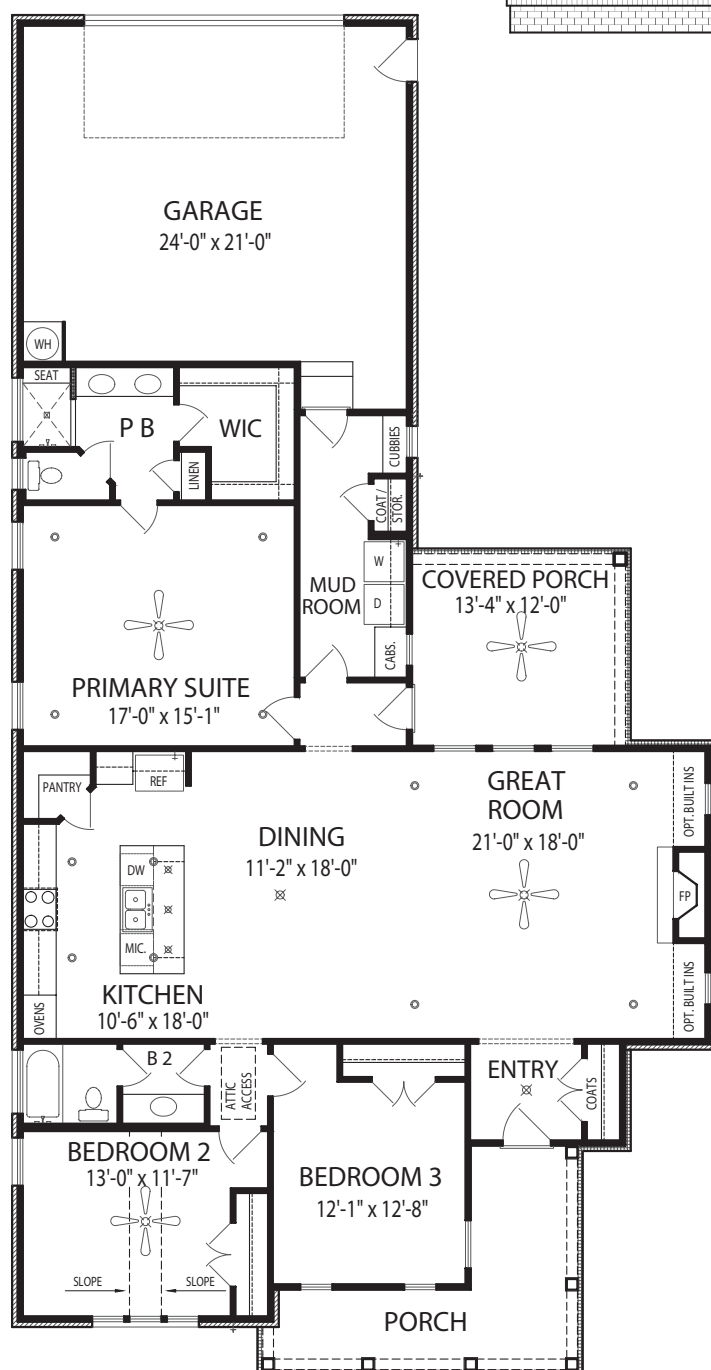
First Level
