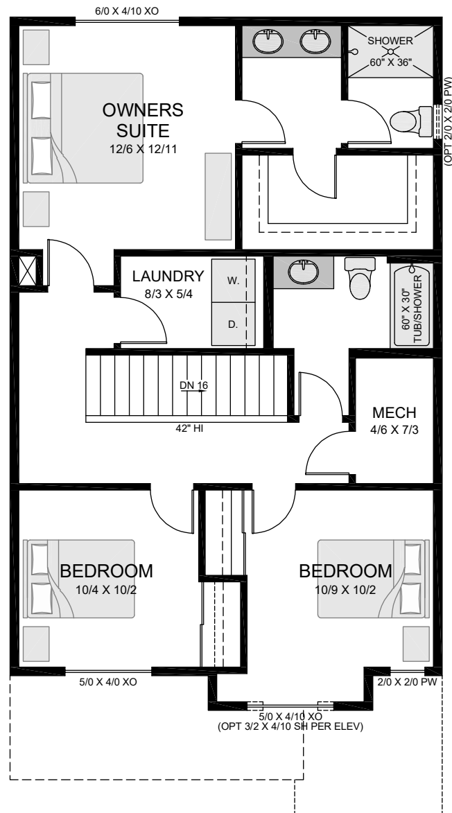
Upper Floor
