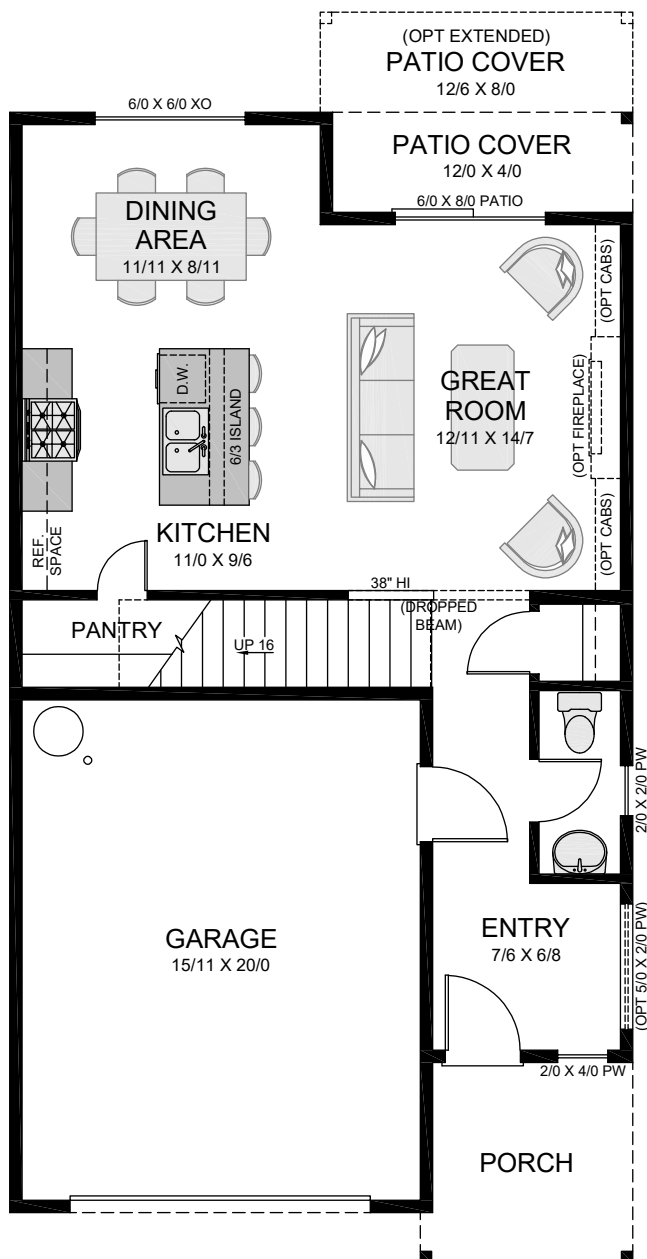
Main Floor
