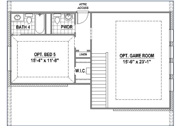
Optional Game Room, Powder Bath & Bedroom 5 with Bath 4 (+791 SF)
