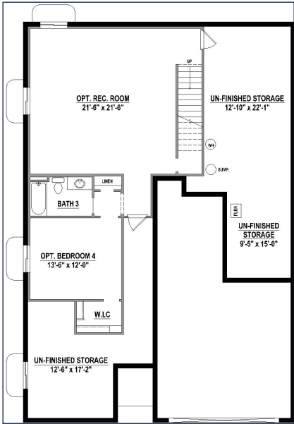
Optional Rec Room with Bedroom 4 & Bath 3 (+945 SF)
