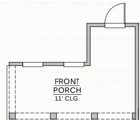
1st Floor Elevation C
