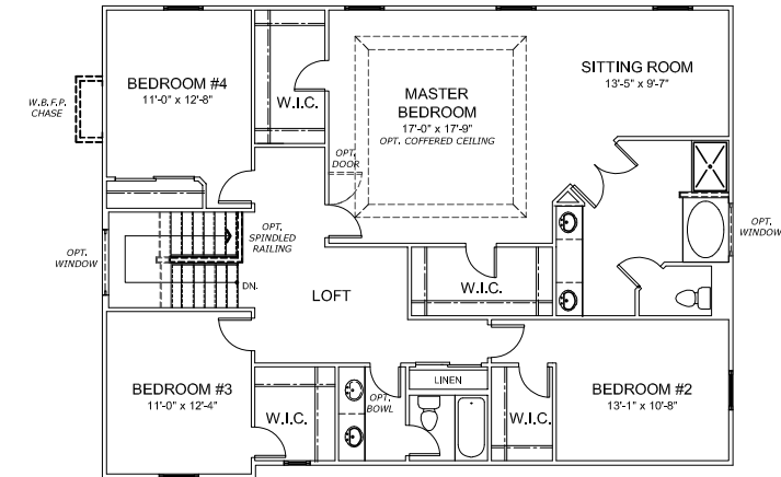
OPT. SECOND FLOOR PLAN
