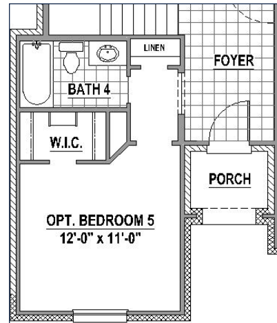
Bedroom 5 w/ Bath 4 ILO Study & Powder Bath
