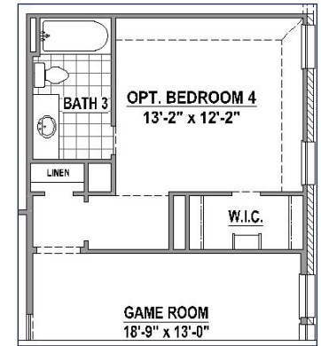
Bedroom 4 w/ Bath 3 (+333 SF)
