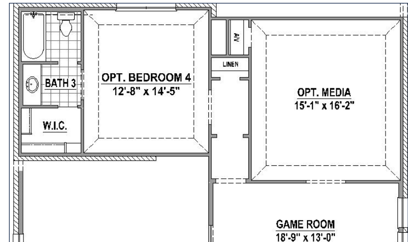
Bedroom 4 w/ Bath 3 & Media Room (+641 SF)
