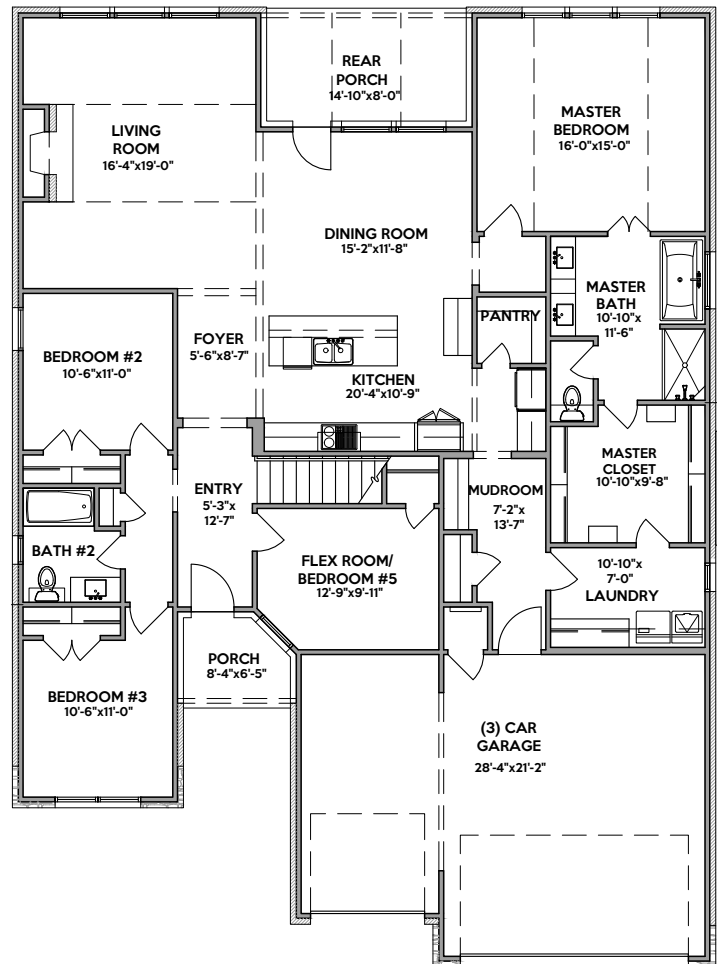
FIRST FLOOR ELEVATION "A", "C" & "D"
