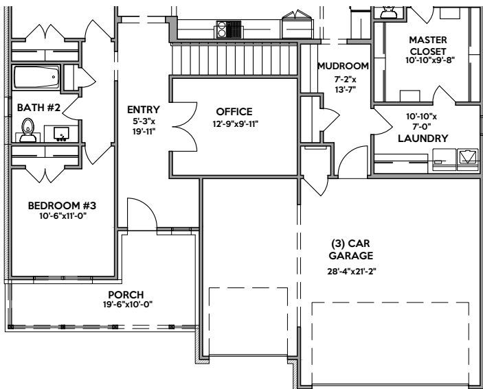
FIRST FLOOR ELEVATION "B" (APPROX. 63 SQ FT MORE)
