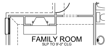
Opt. Fireplace
