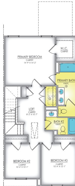
SECOND LEVEL - B-1
