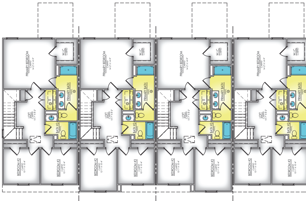
SECOND LEVEL - 4 UNITS
