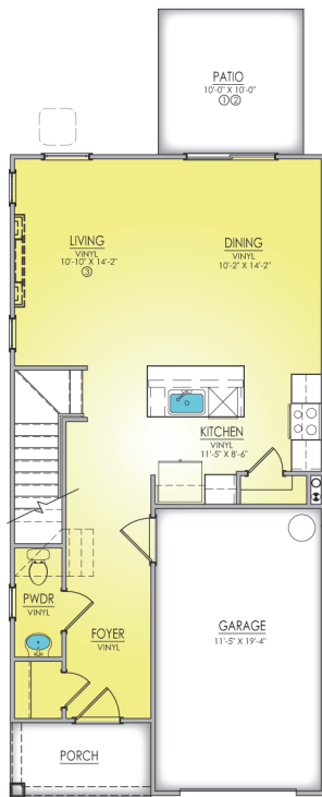
MAIN LEVEL - A-1
