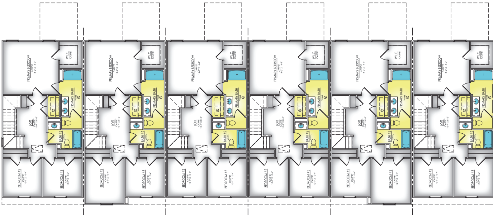
SECOND LEVEL
