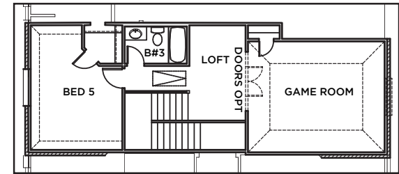
BEDROOM 5, BATH 3 AND GAME ROOM OPT *SECOND FLOOR OPTION
