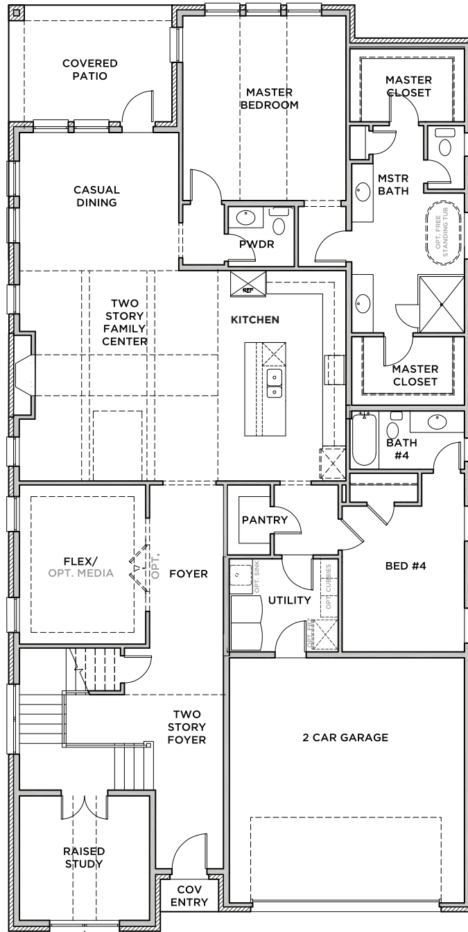
FIRST FLOOR
