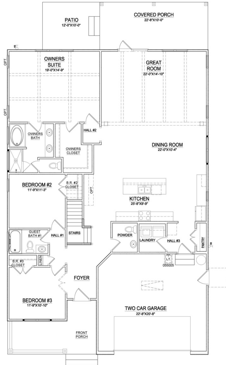
Standard First Floor
