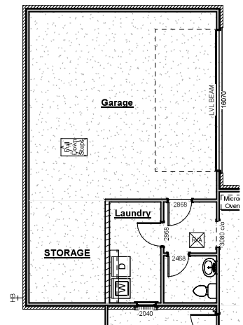
2-Car Garage Storage Addition
