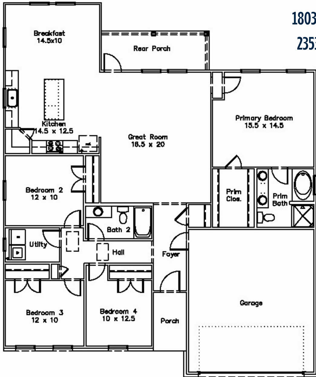
FIRST FLOOR PLAN (48'-5 1/2" x 57'-6 1/2")
