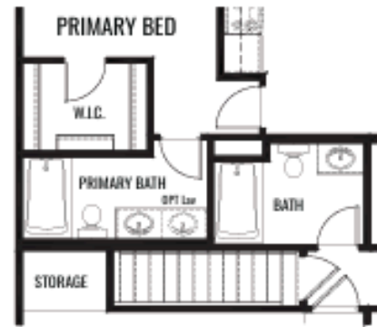
OPTIONAL PRIVATE BATH AT OPTIONAL BASEMENT
