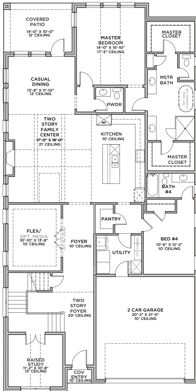
FIRST FLOOR
