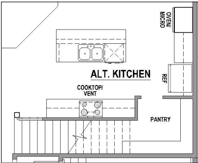
Optional Alternative Kitchen Layout
