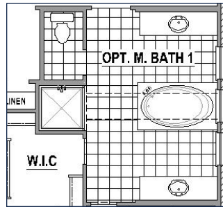
Alternate Main Bath Layout 1 (+93 SF) *not available with Walk-in Pantry & Utility
