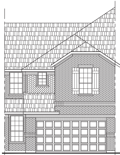
Elevation C
