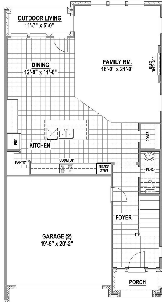
1st Floor
