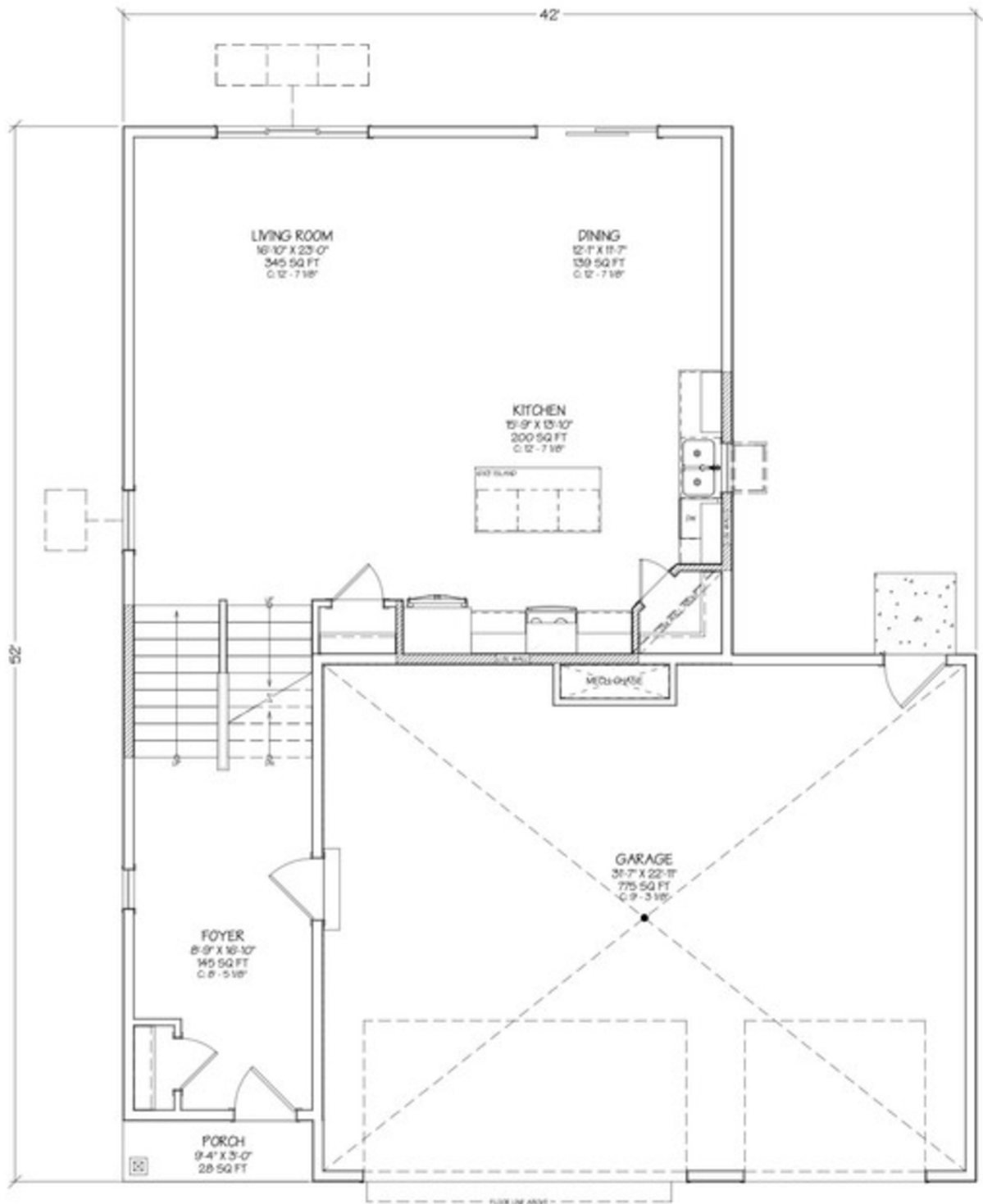
Ava 3.0 - Base Plan - Main Floor - 1,000 sq ft
