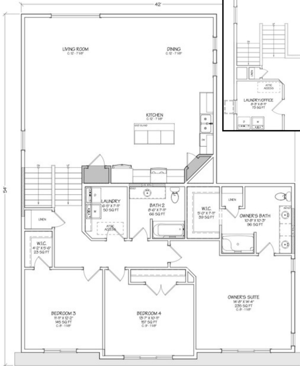
Ava 3.0 - Base Plan - Upper Floor - 1,887 sq ft
