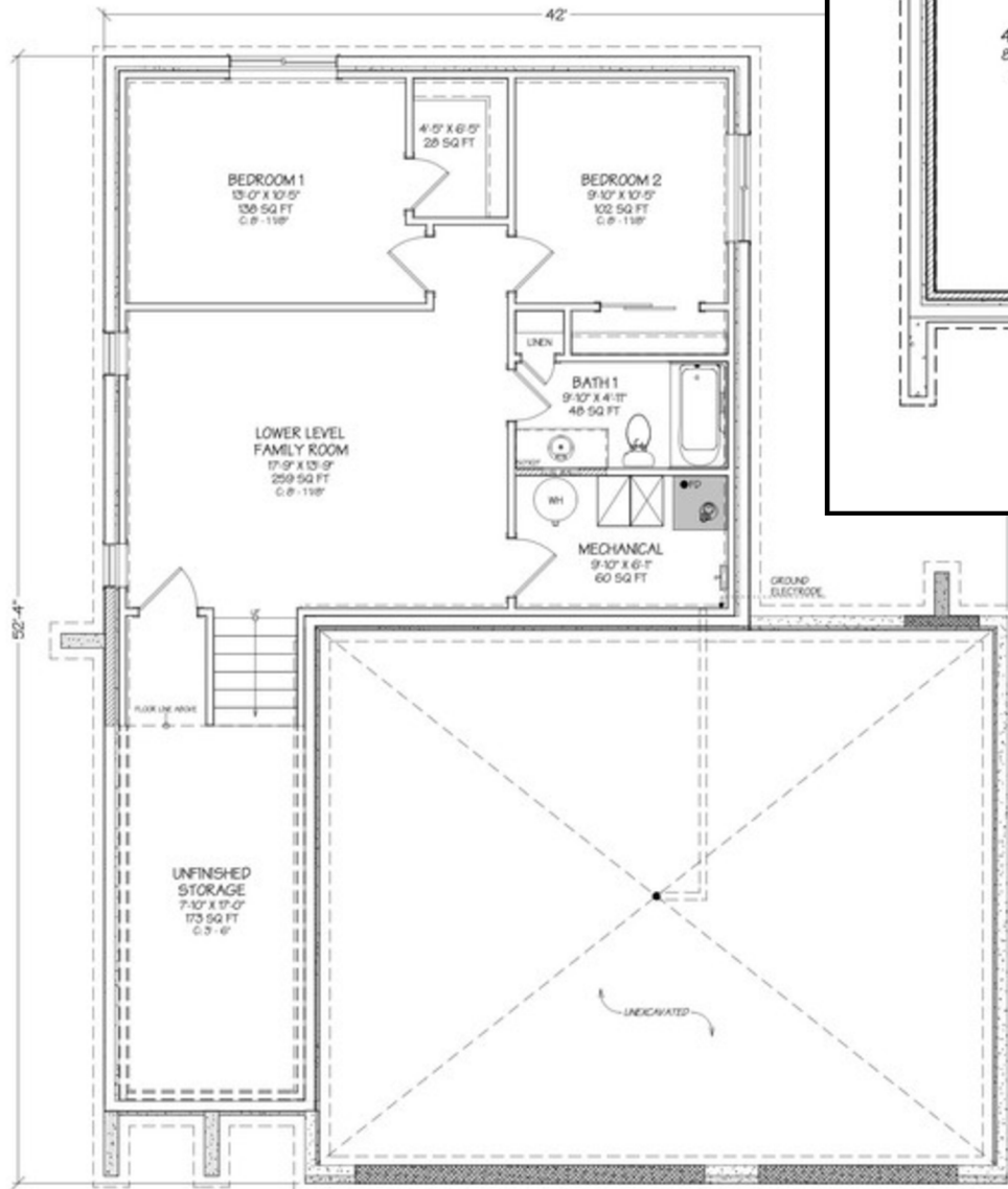
Ava 3.0 - Base Plan - Lower Floor - 1,016 sq ft
