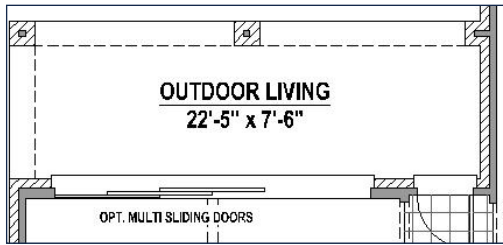
Multi-Sliding Door at Family Room
