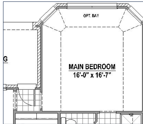
Main Bay Window (+44 SF)
