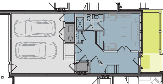
First Floor 51' x 24'
