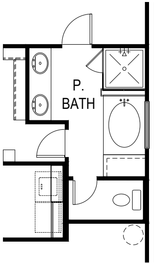
OPTIONAL PRIMARY BATH
