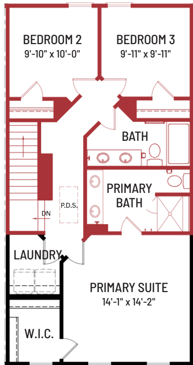
Optional Third Floor Showing 2140 Elevation A
