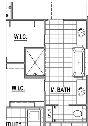
Freestanding Tub at Main Bath
