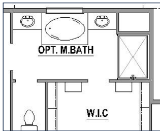
Alternate Main Bath Layout
