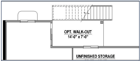
Basement Walkout w/ Deck Above
