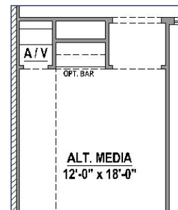
Optional Dry Bar in Media Room
