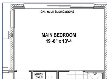
Optional Multi-Sliding Doors in Main Bedroom
