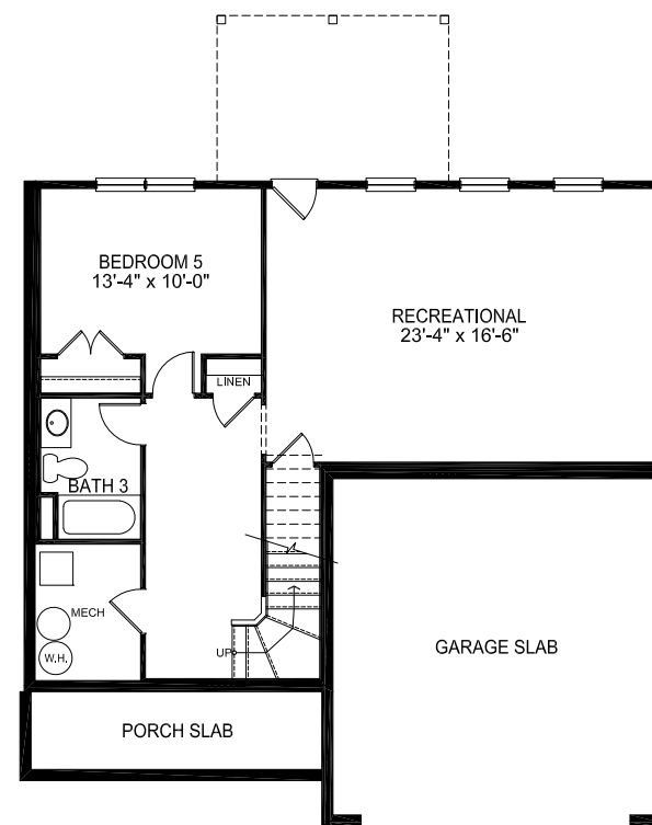
Opt. Basement
