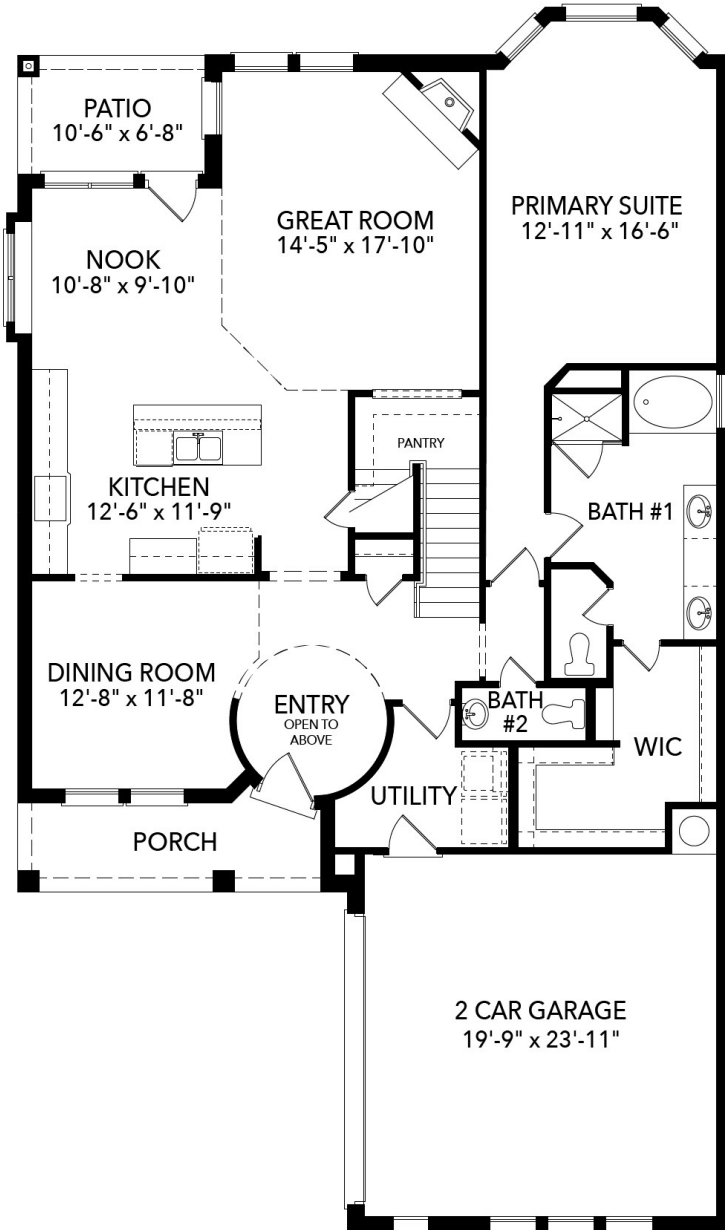
First Floor
