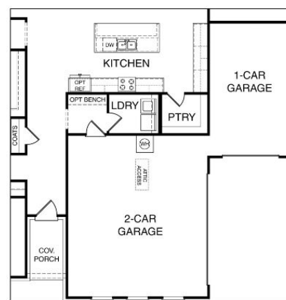
3-CAR SIDE ENTRY GARAGE
