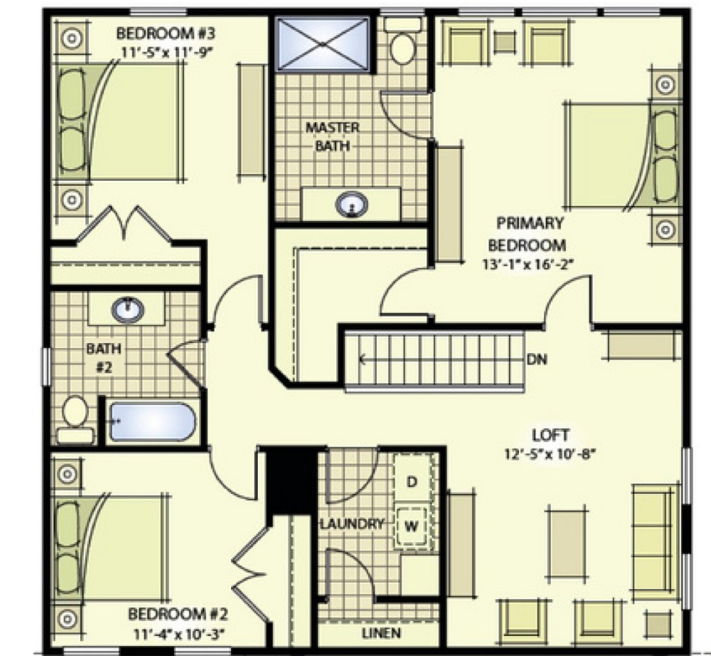
SECOND FLOOR
