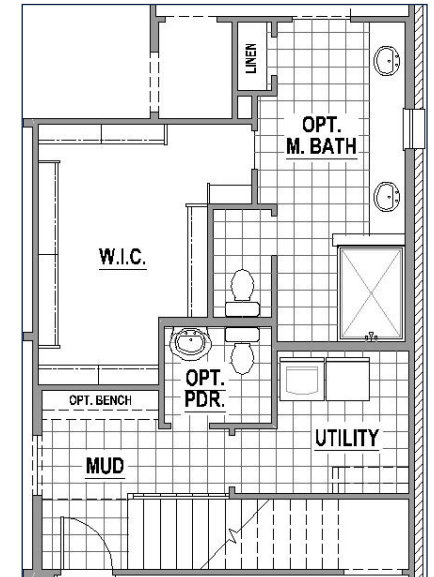
Powder & Alternate Main Bath Layout w/ Stairs to 2nd Floor Options
