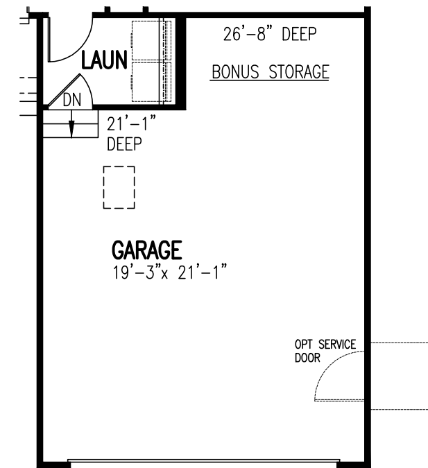
Opt Laundry Room With 6' Garage Extension, Site Permitting
