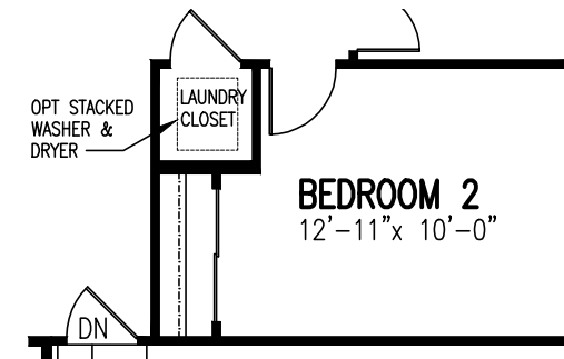
Opt Laundry Closet ilo Coat Closet
