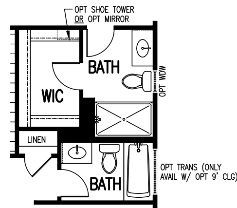
Opt Double Bathroom Layout #1
