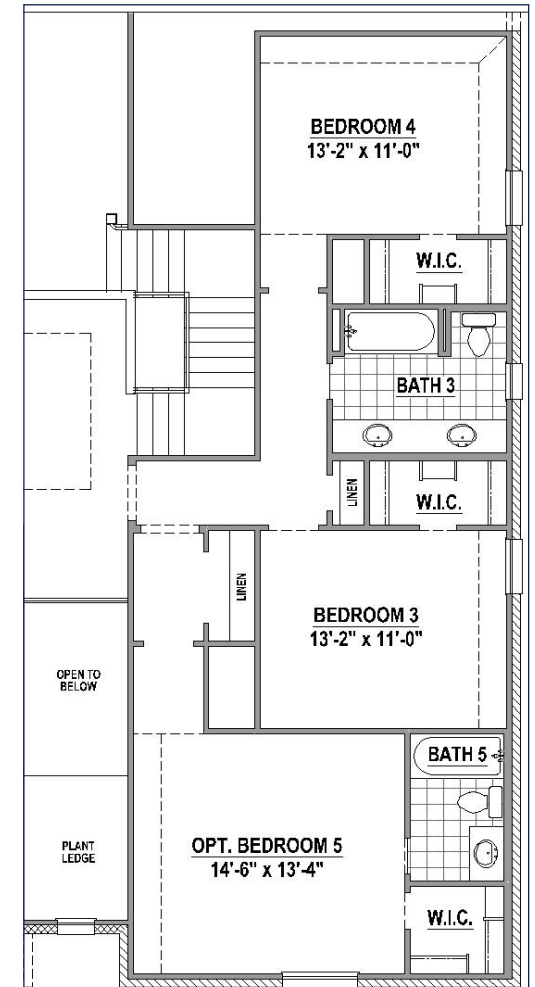
Bedroom 5 w/ Bath (+398 SF)
